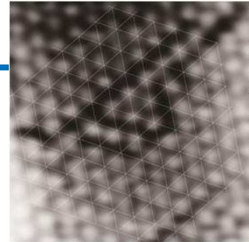
LPSO (Synchronized Long Period Stacking Ordered)相のSTM観察[S. Kurokawa, A. Yamaguchi and A. Sakai, Materials Transactions 54, 1073-1076 (2013)]
